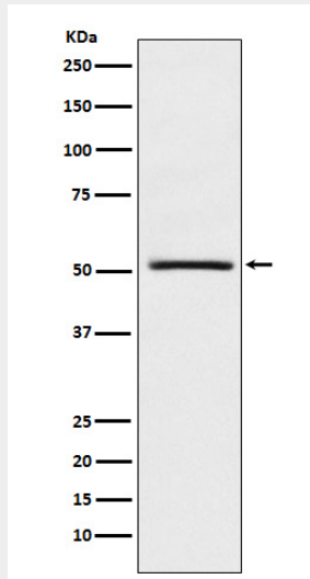
Western blot analysis of NR0B1 / Dax1 expression in A431 cell lysate.
